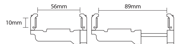
99913 MT-one Smartphone Tripod Kit Set
