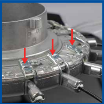
Collapsed the Softbox, push the button to release the rod locked
